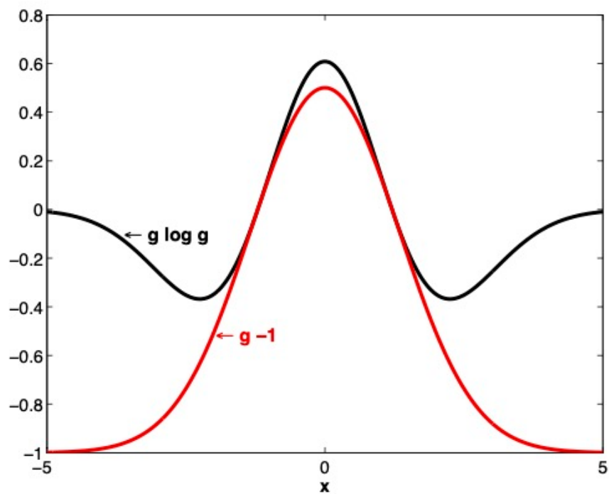
Fig. 25.3: Graphs of g \log g and g - 1 where g is the ratio of the density of a \mathcal{N}(0, 1) random variable to the density of a \mathcal{N}(0, 1.5) random variable. Under the \mathcal{N}(0, 1.5) density, Eg = 1 .
