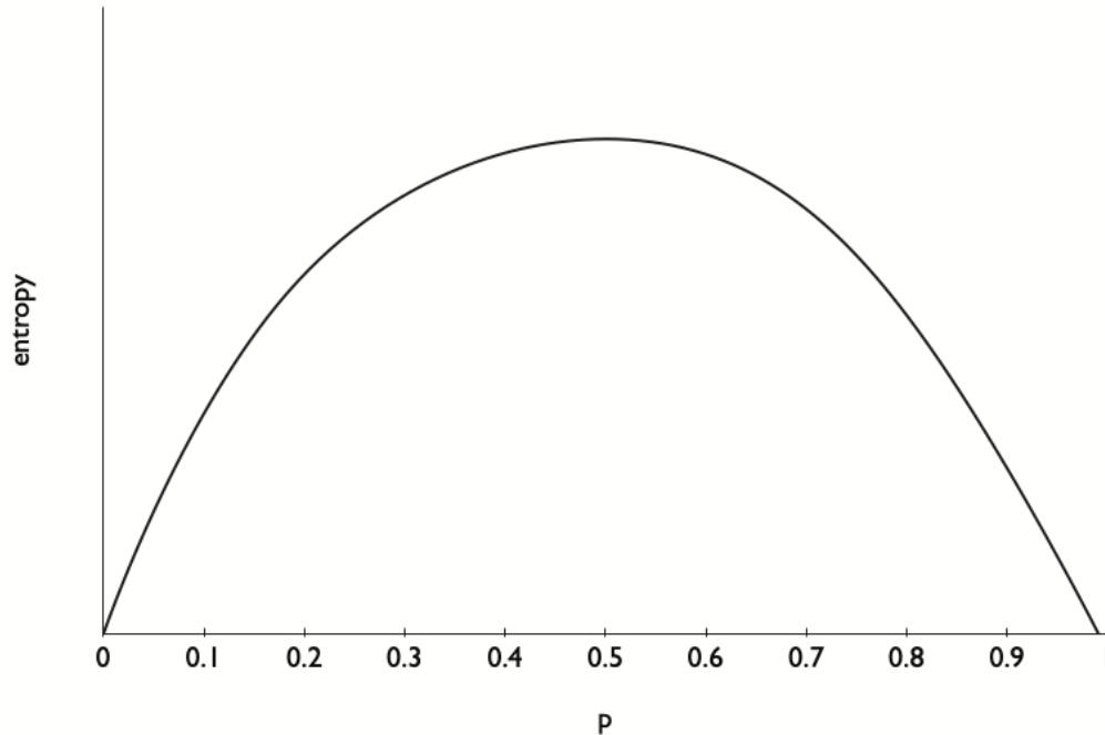
Fig. 25.1: Entropy as a function of \hat{\pi}_1 when \pi_1 = .5 .
