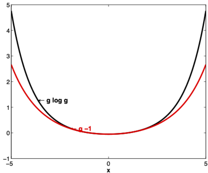
Fig. 25.4: g \log g and g - 1 where g is the ratio of the density of a \mathcal{N}(0, 1) random variable to the density of a \mathcal{N}(0, 1.5) random variable. Under the \mathcal{N}(0, 1.5) density, Eg = 1 .
