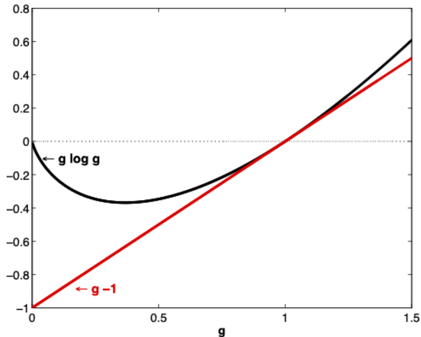
Fig. 25.2: The function g \log g for g \geq 0 . For a random variable g with Eg = 1 , Eg \log g \geq 0 .
